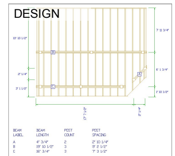
3D DECK+RAIL DESIGN
